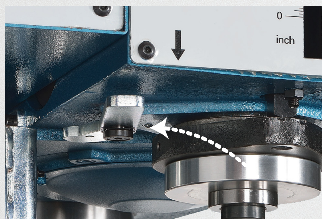
Release handle. Easy release of the drill without using of tools.
